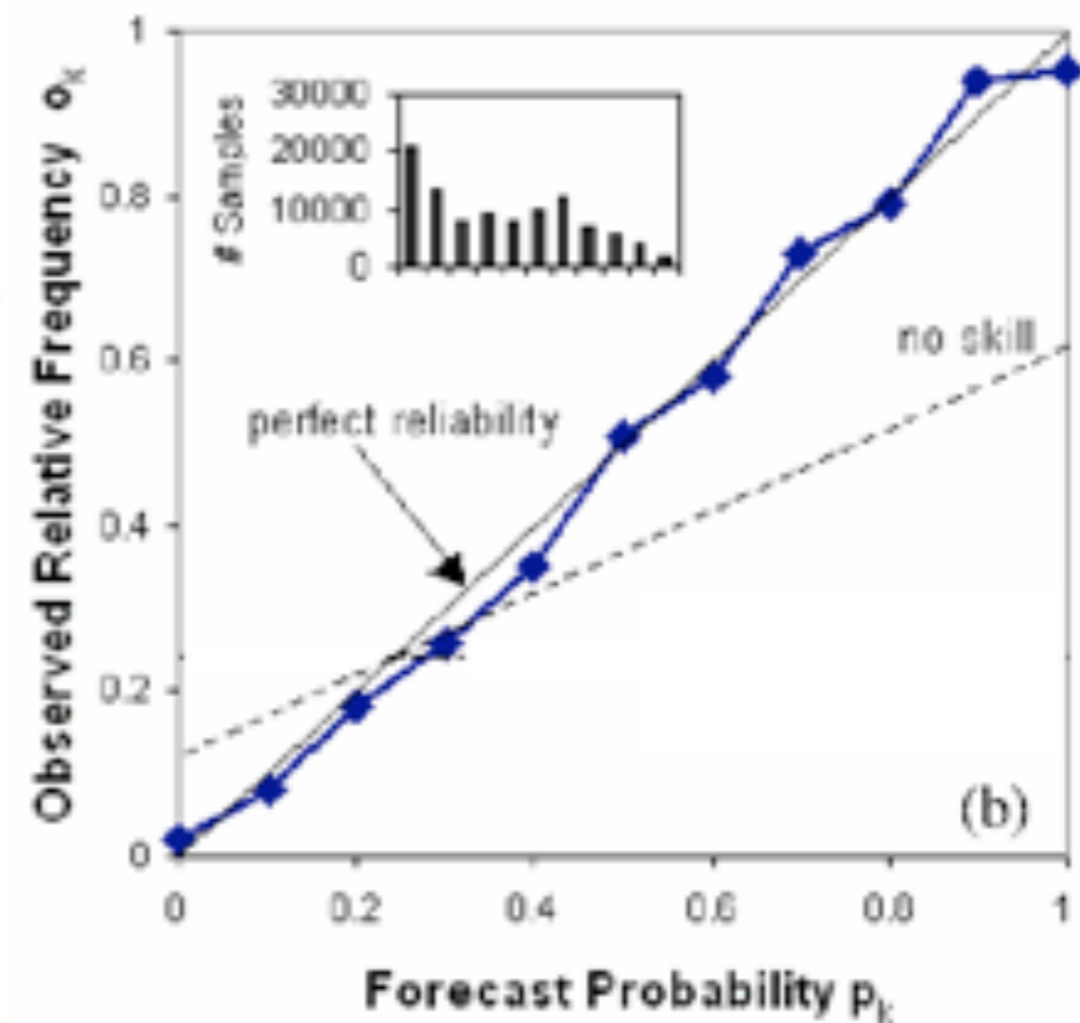
Reliability Diagram
