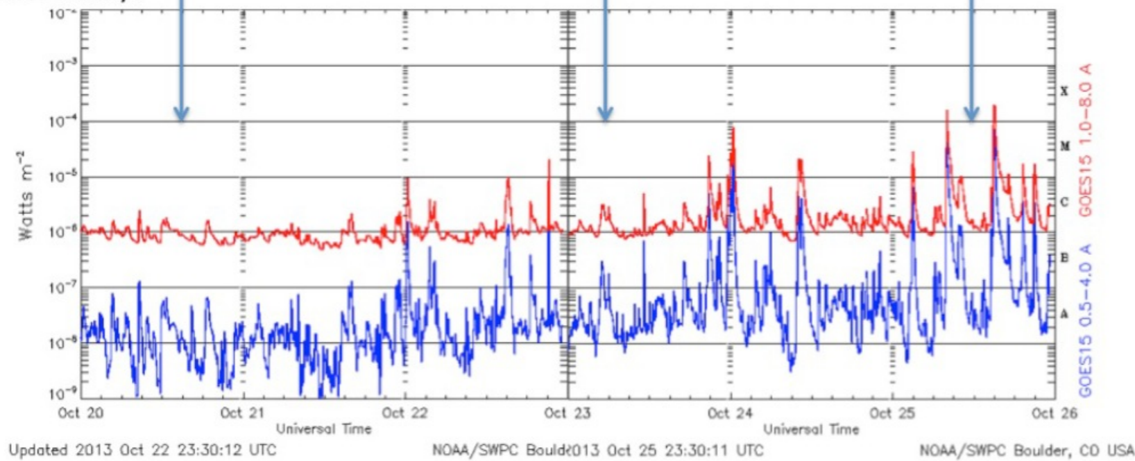
(b) GOES X-rays
